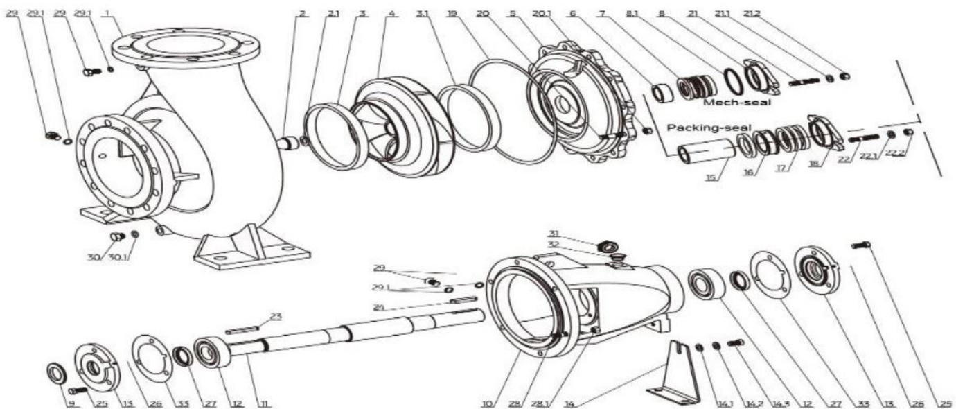
Despiece kit
