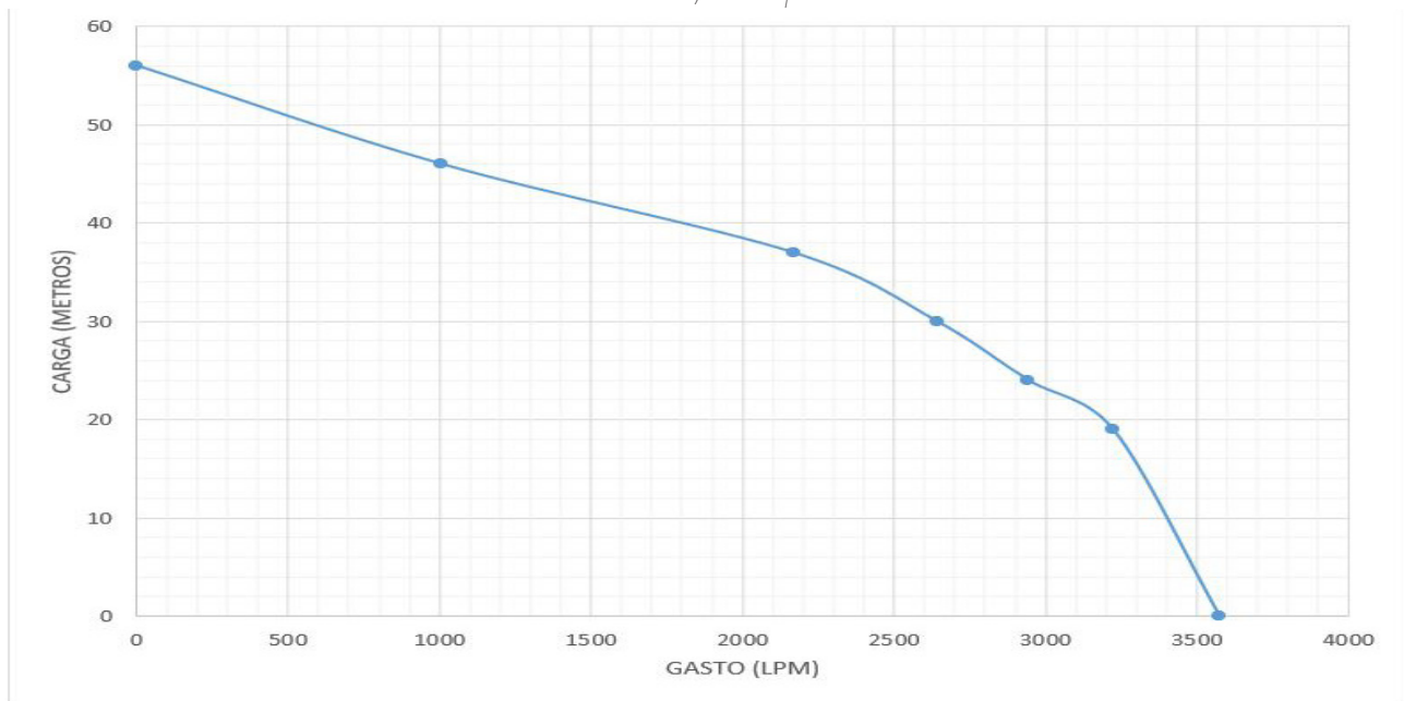
Curva a 3,000 rpm.
